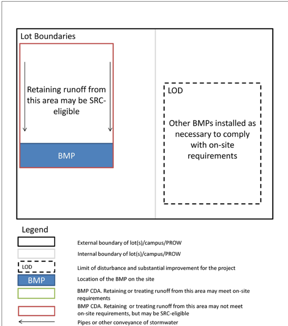
Figure UY.18 Many lots: BMP and CDA are on an adjacent, undisturbed lot.
