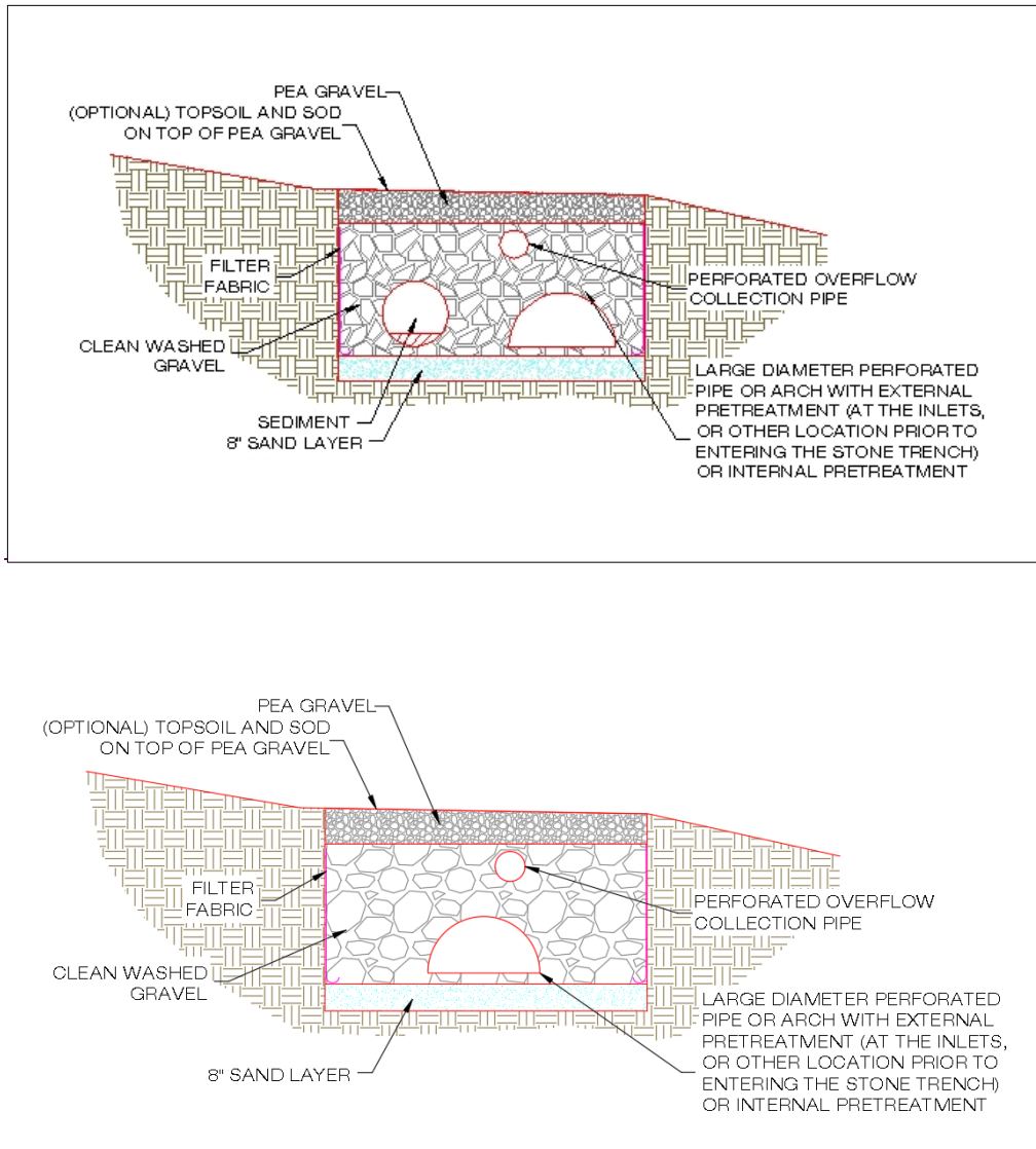
Figure 3.33-34 Infiltration section with supplemental pipe storage.
