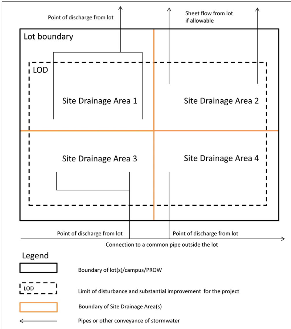
Figure UW.1 Site Drainage Areas on a single lot.
