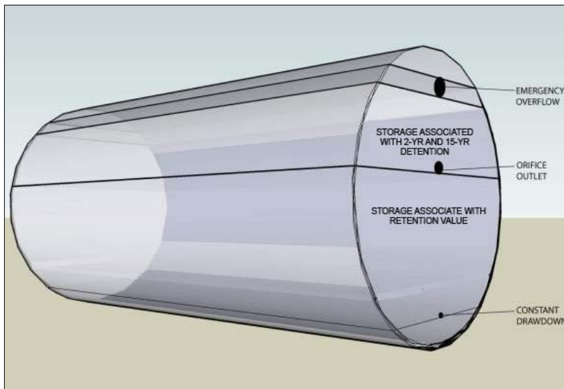
Figure 3.8-9 Cistern Design 3: Constant drawdown version where storage is associated with design storm, channel protection, and flood volume.
