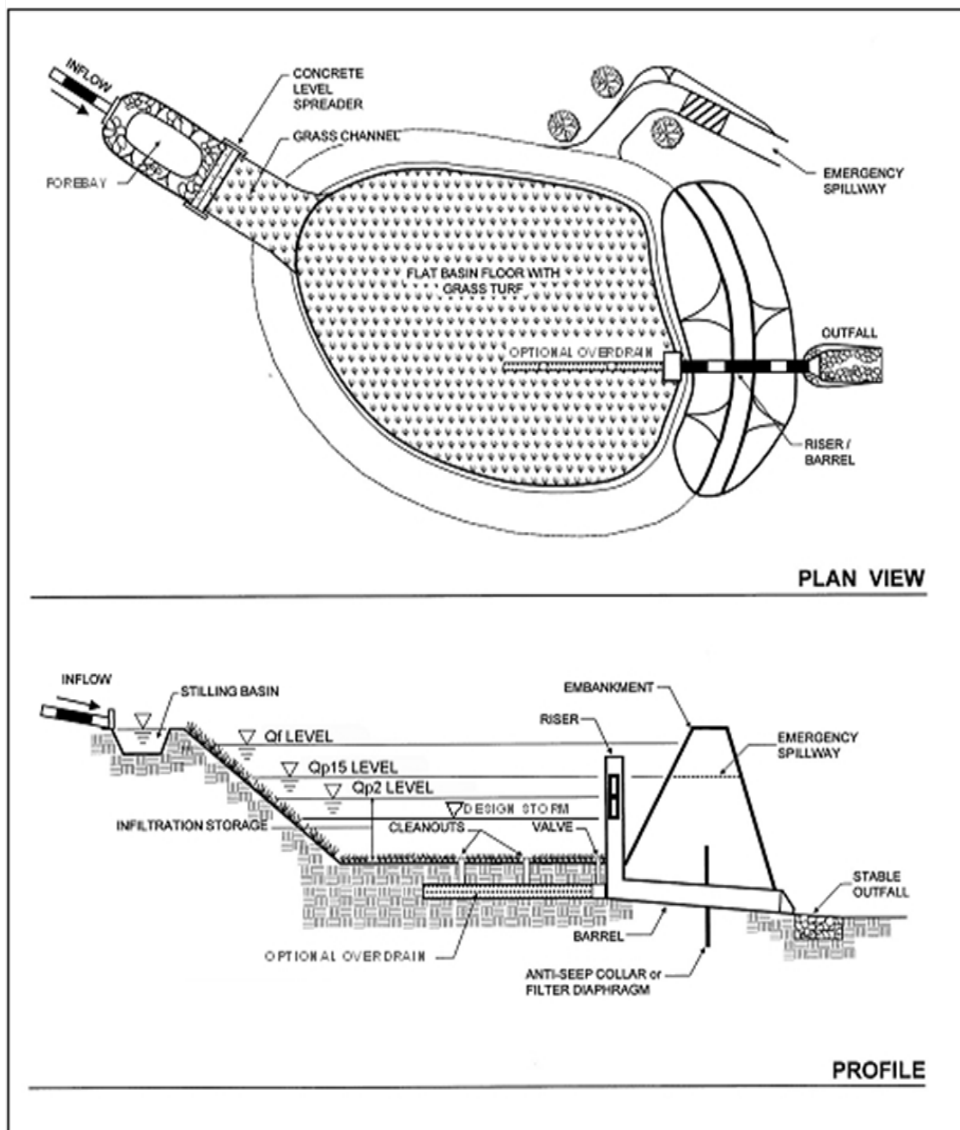
Figure 3.34_35 Example of an infiltration basin.
